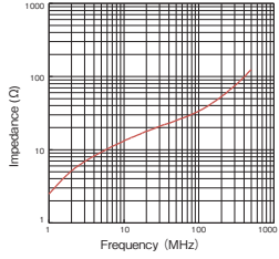
GTR-13-7-6
