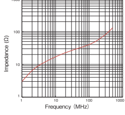
GTR-16-10-7
