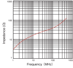
GTR-14-5-10-8
