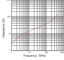
GTR-18-10-6
