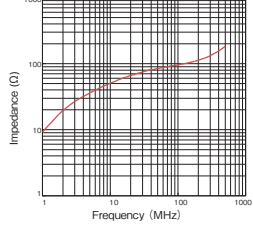
GTR-20-10-10
