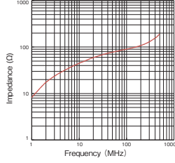
GTR-31-19-8
